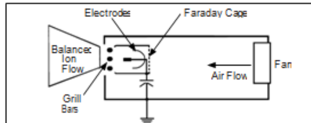
Figure 6. Components of the Faraday Balance System
